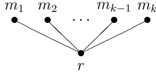
FIGURE 4. The k -fork \mathfrak{F}_k .
