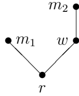
FIGURE 5. The tree \mathfrak{F} .
