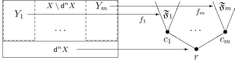
FIGURE 9. Depiction of f : X \rightarrow \mathfrak{F} .
