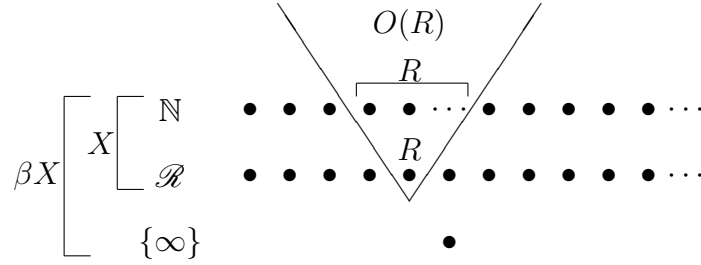
FIGURE 3. Depiction of \beta X = \alpha X for a Mrowka space X , and of O(R) for R \in \mathcal{R} .
