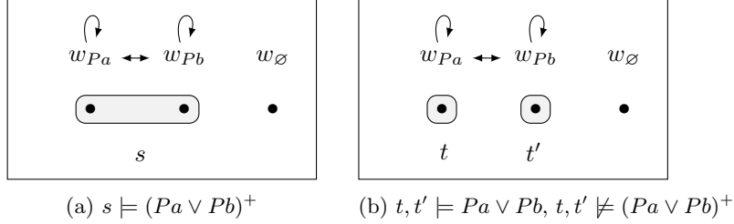
Figure 2: Ignorance inference follows from pragmatic enrichment
