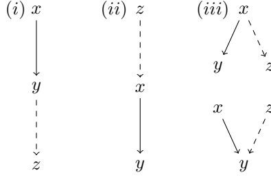
Figure 1: Illustration of Definition 23, indicating given edges (solid) and implied edges (dashed).
