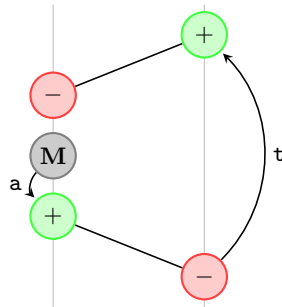
Fig. 9. The plot unit structure for (12).
