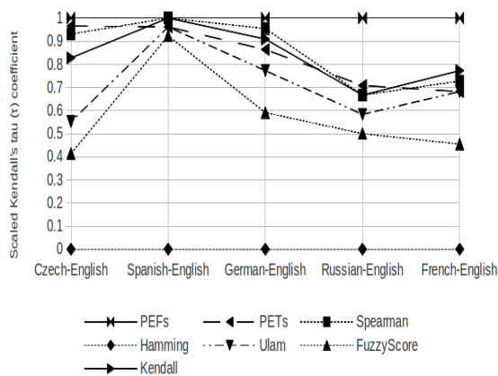
Figure 10: Plot of scaled Kendall tau correlation for translation into English
