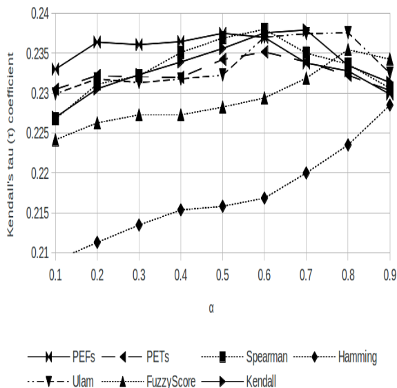
Figure 7: Effect of \alpha on German-English evaluation for \beta = 0.6
