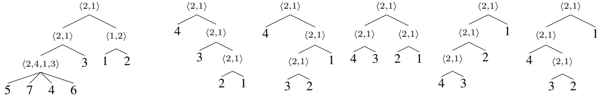
Figure 3: A PET for \pi = \langle 5, 7, 4, 6, 3, 1, 2 \rangle . And five different PETs for \pi = \langle 4, 3, 2, 1 \rangle .
