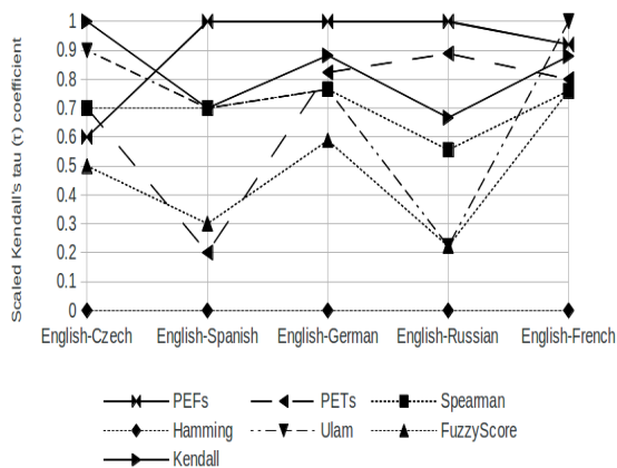
Figure 9: Plot of scaled Kendall tau correlation for translation from English
