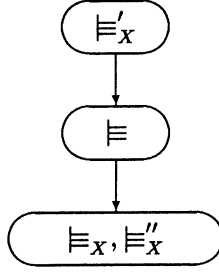
Figure 2: Overview of the implication definitions
