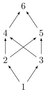
A partial order
