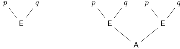
Figure 6: Failure of idempotence.
