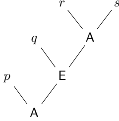
Figure 3: A three-step game
