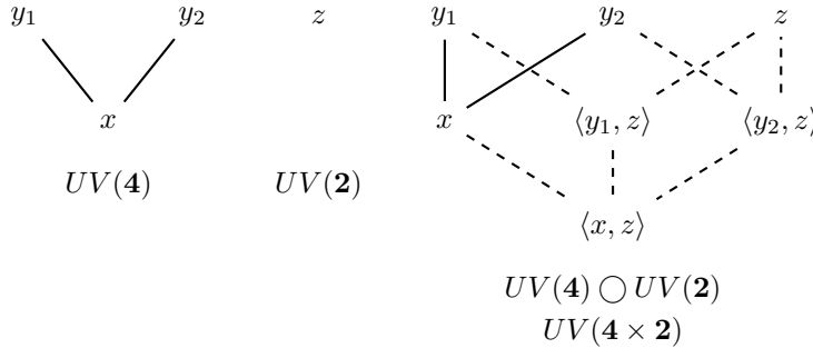
FIGURE 2. UV-sum of the UV-duals of the BAs 4 and 2 .
