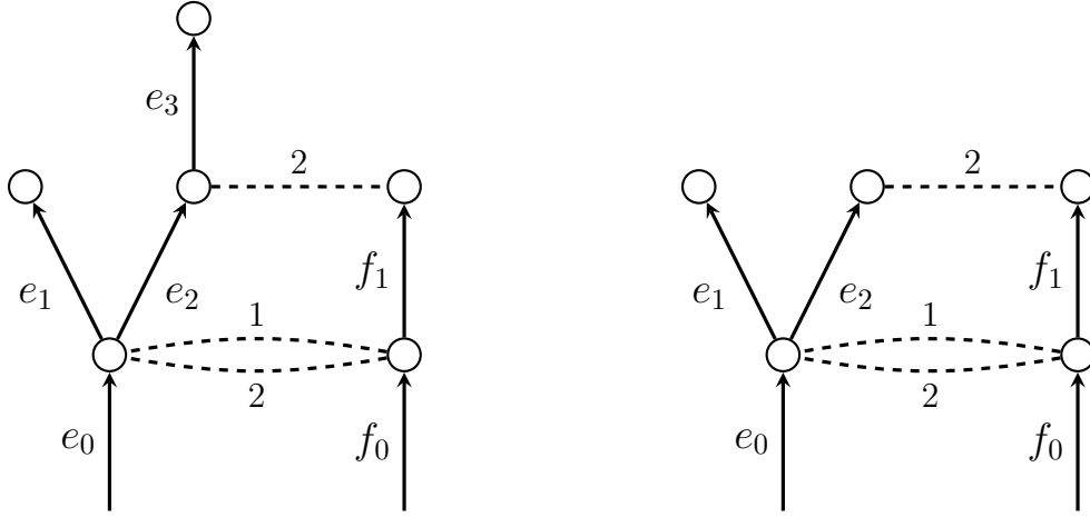
Figure 1.5: ETL Models
