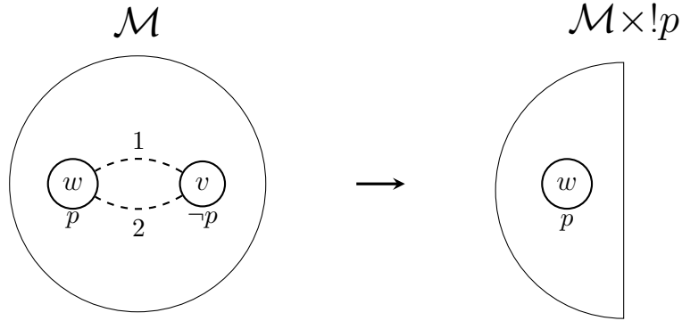
Figure 1.2: Public Announcement
