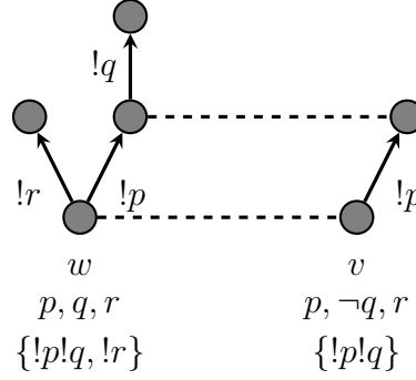
Figure 4.1: TAPAL with Verificationist Interpretations
