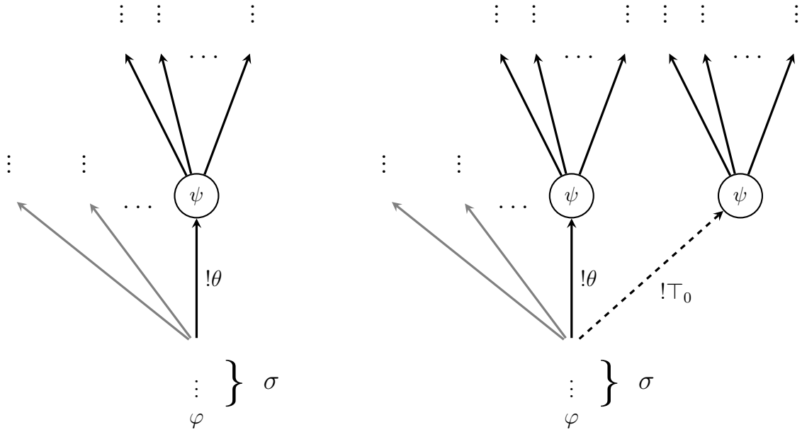
Figure 3.4: Grafting Subtrees
