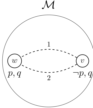
Figure 1.1: Epistemic Model
