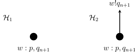
Figure 3.2: TAPAL-Model 2
