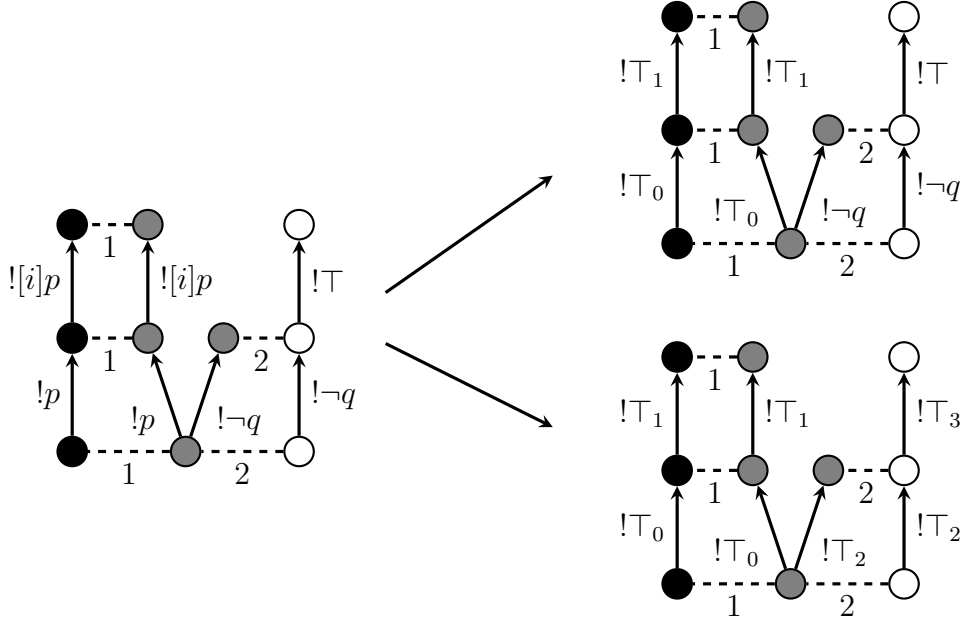
Figure 2.1: Model Normalization
