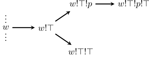
Figure 3.1: TAPAL-Model 1
