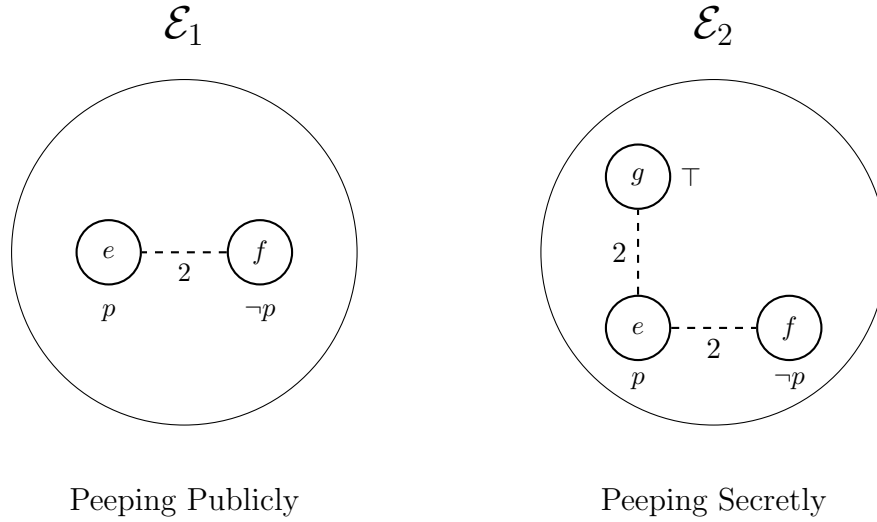
Figure 1.3: Event Models
