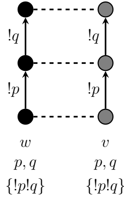
Figure 5.2: Counterexample
