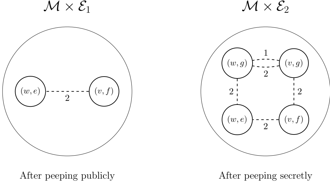
Figure 1.4: Product Update
